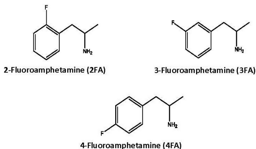
Figure 1. 2FA, 3FA and 4FA structures
