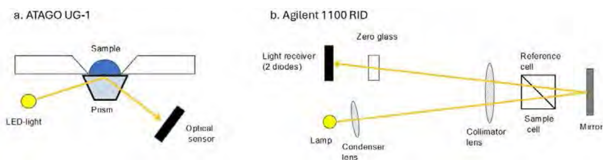
Figure 1. Detection principle of a) Atago UG-1 digital refractometer and b) Agilent 1100 RI-detector
