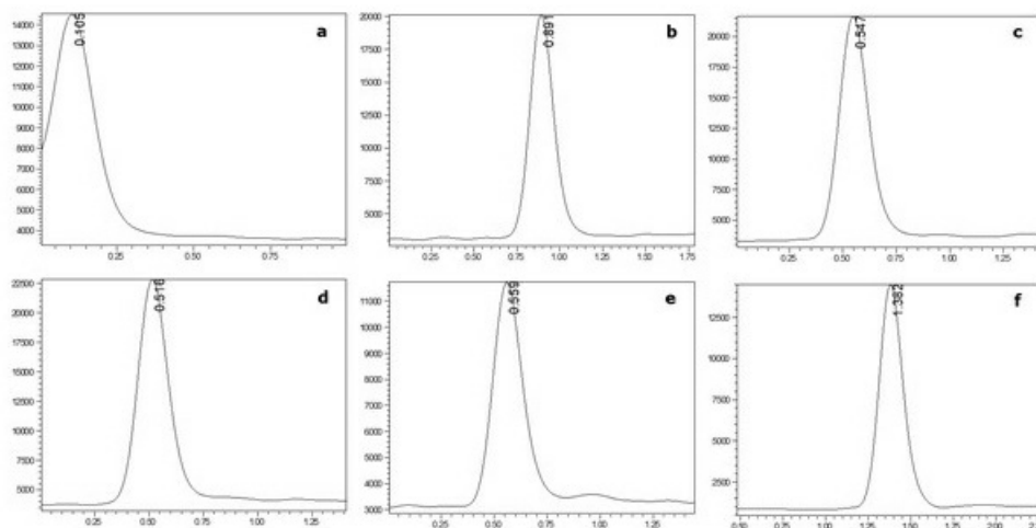
Figure 1. Single-ion ( m/z = 45.0 ) chromatograms of CD 3 CN for (a) zero-volume union; (b) CORTECS T3 C18 (100 \times 3.0 mm, 2.7 \mu m); (c) Zorbax Eclipse Plus C18 (100 \times 2.1 mm, 1.8 \mu m); (d) Poroshell 120 (100 \times 2.1 mm, 2.7 \mu m); (e) LUNA C18 (100 \times 2.0 mm, 3 \mu m); and (f) ODS Hypersil (60 \times 4.6 mm, 3 \mu m) columns. Mobile phase: 0.01 % formic acid in acetonitrile; flow rate: 0.5 mL/min; injection volume: 20 \mu L.
