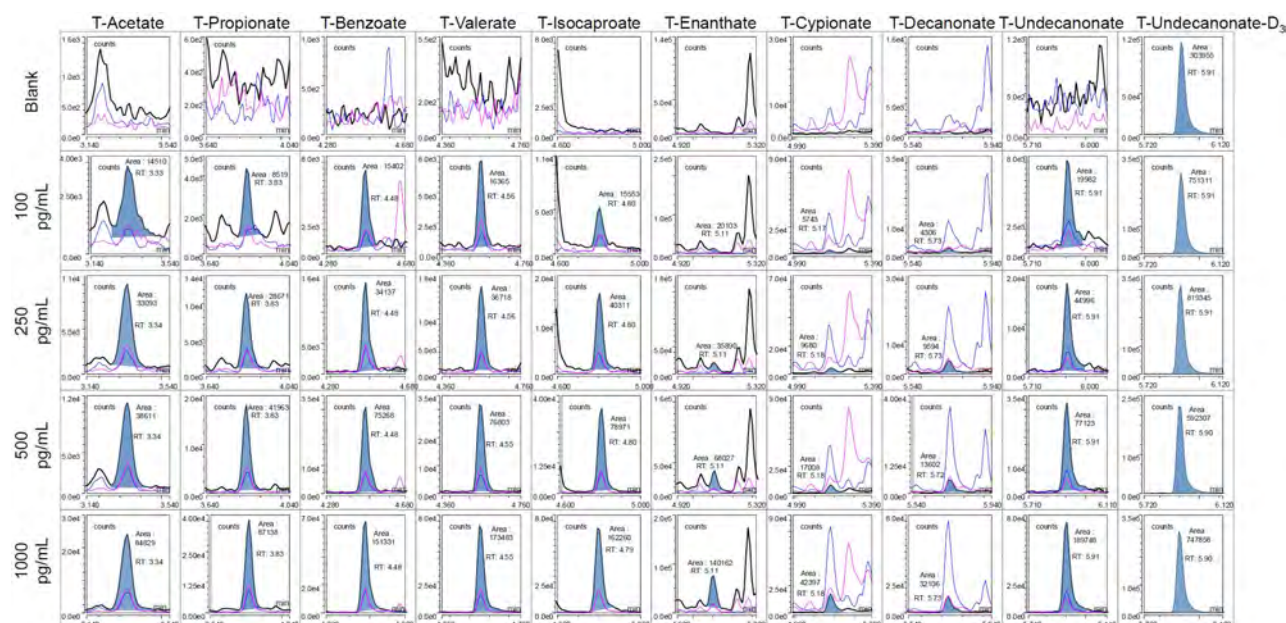
Figure 2. SRM chromatographs on TSQ Altis Plus for an extracted blank DBS at various spiked concentrations of testosterone esters
