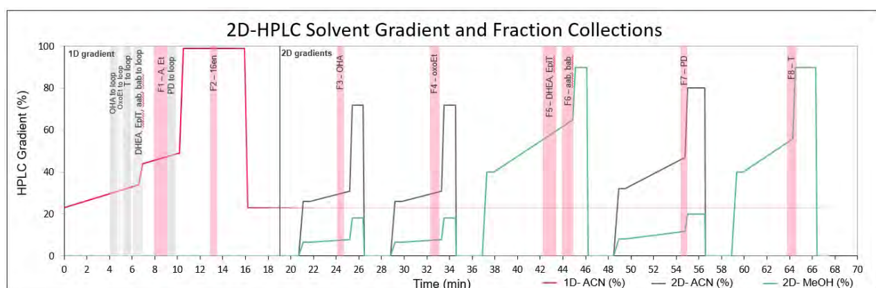
Figure 2. HPLC solvent gradient and collection windows for the 2D cleanup procedure. Column 1: Phenomenex Kinetix 2.6 \mu m Phenyl-Hexyl 100 Å, 150 mm x 4.6 mm - 1 mL/min; Column 2: Phenomenex Onyx Monolithic HD-C18 130 Å, 100 mm x 4.6 mm - 3 mL/min
