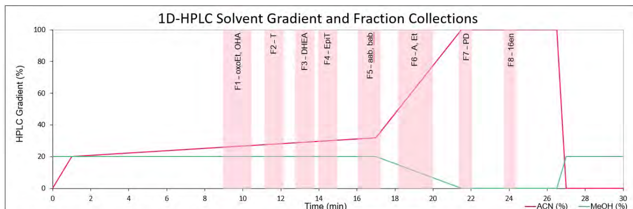
Figure 1. HPLC solvent gradient and collection windows for the 1D cleanup procedure. Column: Phenomenex Kinetix 5 \mu m C18 100 Å, 250 mm x 4.6 mm - 1.2 mL/min Abbreviations: oxoEt: 11-oxoetiocholanolone, OHA: 11 \beta -hydroxyandrosterone, T: testosterone, DHEA: dehydro-epiandrosterone, EpiT: epitestosterone, aab: 5 \alpha -androstane-3 \alpha ,17 \beta -diol, bab: 5 \beta -androstane-3 \alpha ,17 \beta -diol, A: androsterone, Et: etiocholanolone, PD: pregnanediol, 16en: 16(5 \alpha )-androstene-3 \alpha -ol
