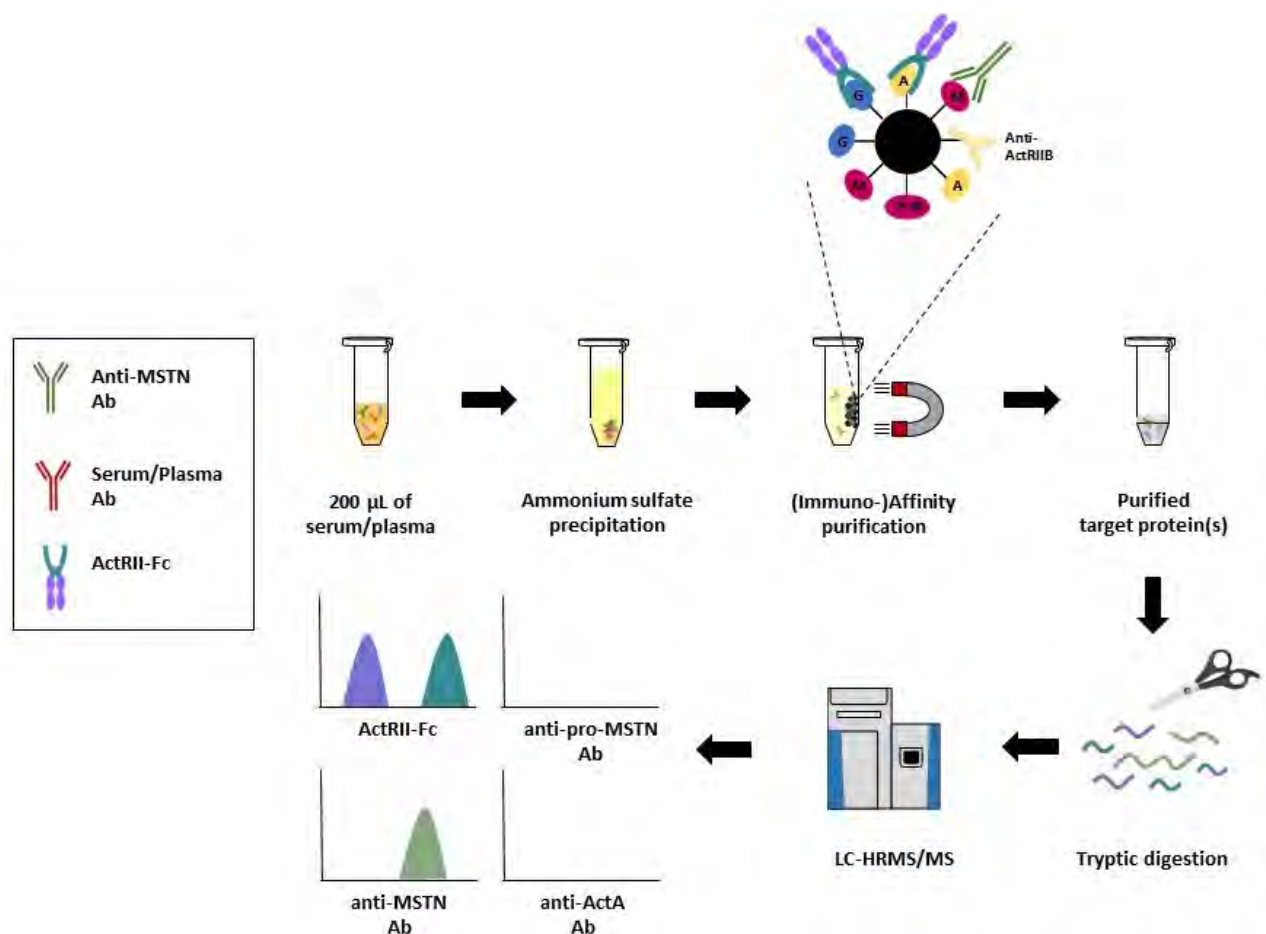
Figure 1. Method overview
