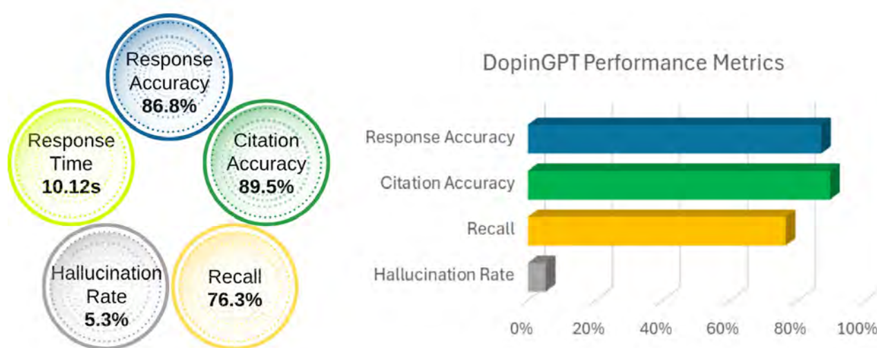
Figure 1. Performance Metrics of the DopinGPT Chatbot: This graphic presents key performance indicators used to evaluate the effectiveness of DopinGPT in supporting doping control operations
